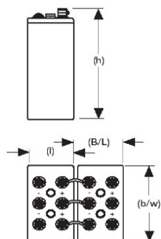
Dimension figure
