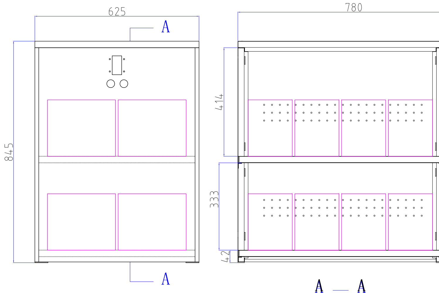
EverExceed 16pcs ST-1280 Battery Cabinet
